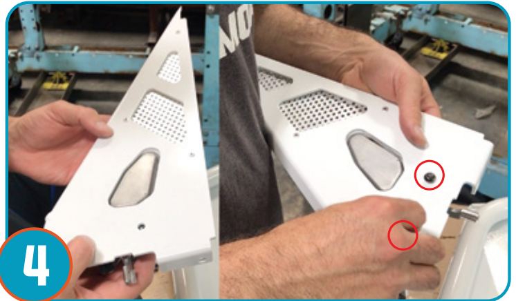
Attach the paddle latch to latch plate as shown with 2 provided bolts. Repeat for opposite door.
