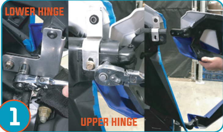
Remove stock door by removing 4 bolts per door and remove lower & upper hinge to remove door from vehicle. Repeat for opposite door.
